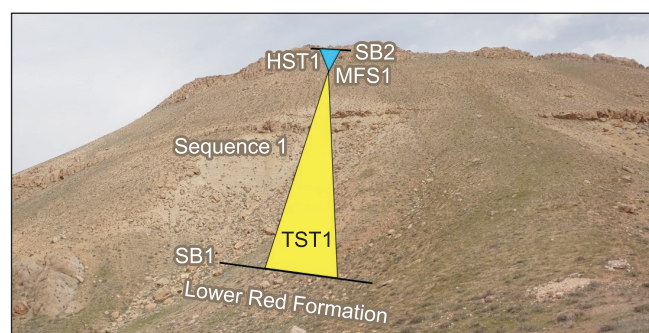
Fig. 9. Outcrop view of the first depositional sequence in the Nowbaran area.
