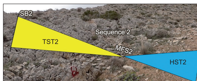
Fig. 10. Outcrop view of the second depositional sequence in the Nowbaran area.
