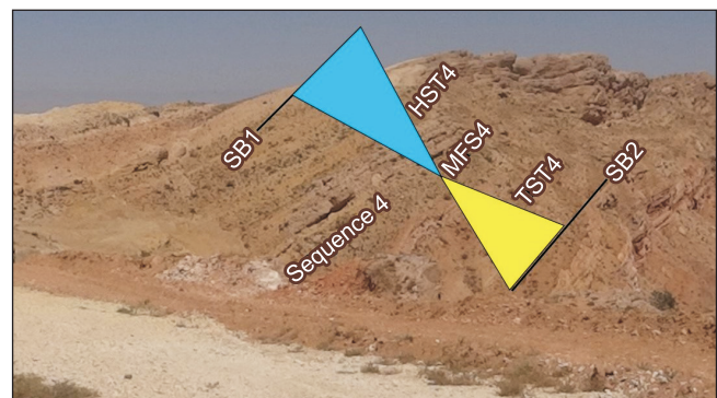
Fig. 13. Outcrop view of the fourth depositional sequence in the Andabad area.
