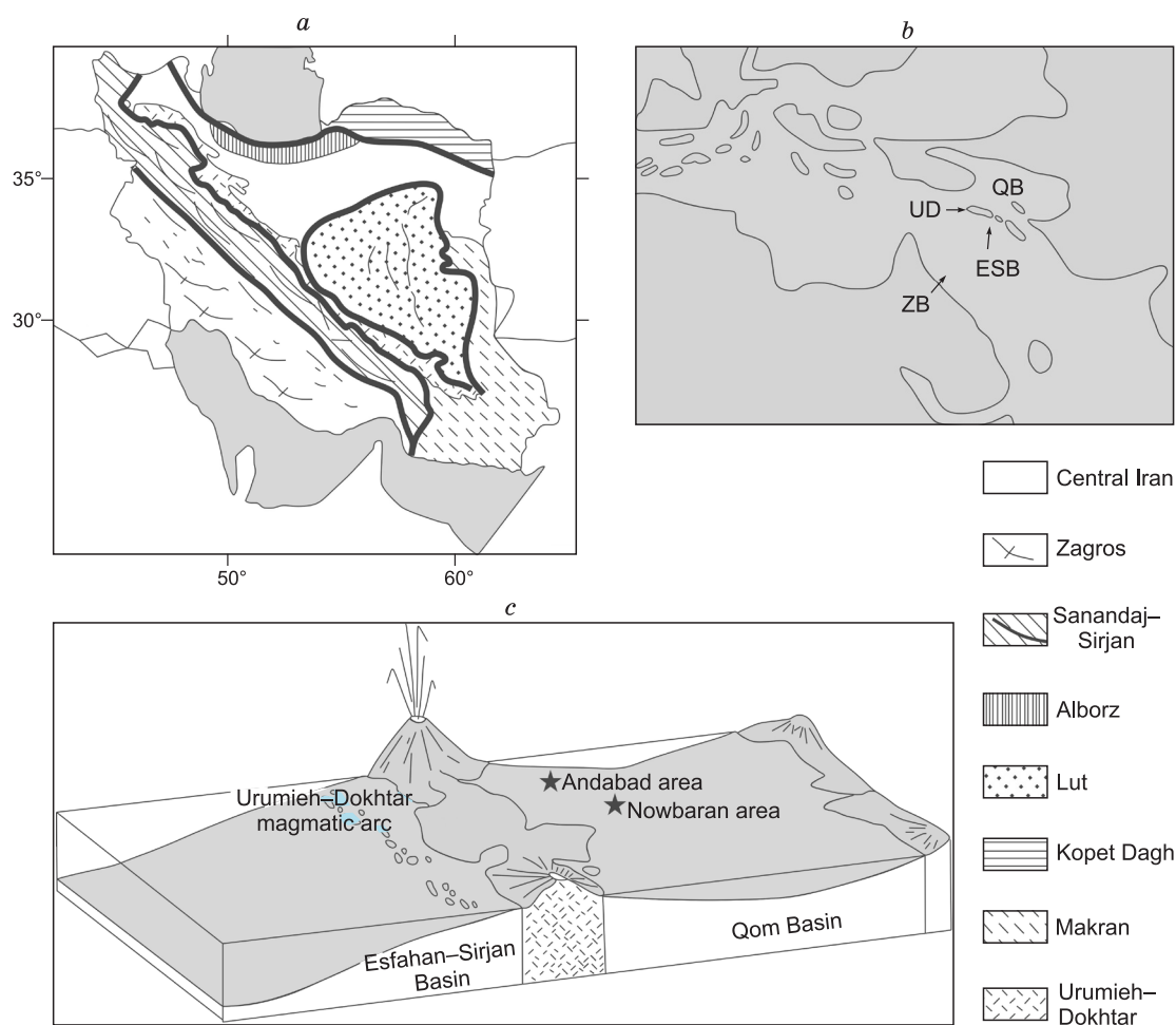
Fig. 1. Paleogeographic setting of the studied area. a , Eight structural-sedimentary zones introduced by Heydari (2008); b , paleogeography map of the Tethyan seaway in Miocene (QB, Qom sub-basin; ESB, Esfahan–Sirjan sub-basin; UD, Urumieh–Dokhtar; ZB, Zagros Basin) (modified from (Harzhauser and Piller, 2007; Reuter et al., 2009)); c , schematic block diagram for the Esfahan–Sirjan and the Qom basins in the early Miocene time (modified from (Reuter et al., 2009)).
