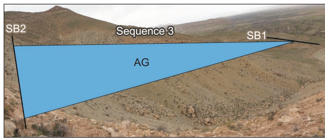
Fig. 11. Outcrop view of the third depositional sequence in the Nowbaran area.
