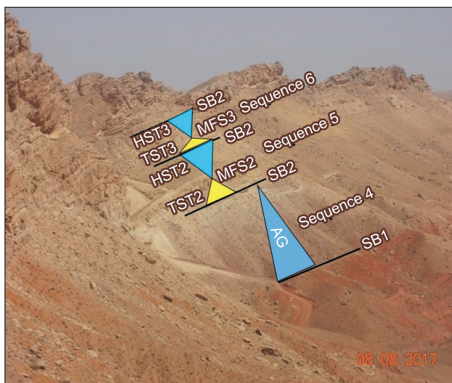
Fig. 12. General view of the first, second, and third depositional sequence in the Andabad area.
