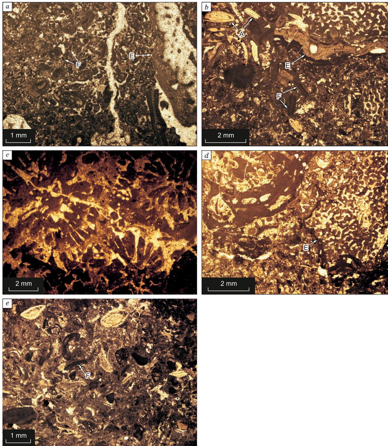
Fig. 4. Taphofacies of the Qom Formation in the Andabad area. a , MTF-1; b , MTF-2; c , MTF-3; d , MTF-4; e , MTF-5. F, Fragmentation; E, encrustation; A, abrasion.
