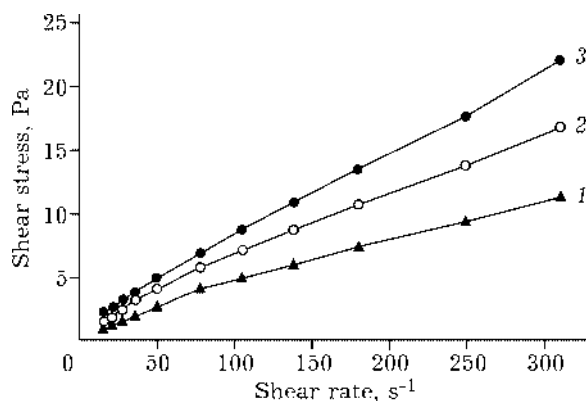
Fig. 5. Flow curves of suspensions: 1-3 - samples 1-3, respectively.
