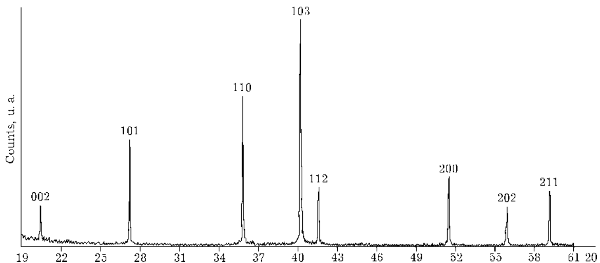
Fig. 5. End products identification: XRD analysis \text{CuK}\alpha ( \lambda = 0.139 nm) for the G5(350/250/3 h) ball milling condition.
