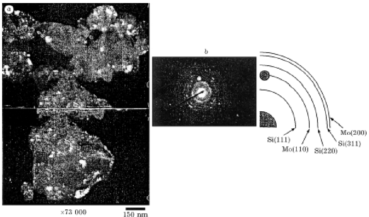
Fig. 3. TEM observation of as-milled powder particles from G5(350/250/3 h) condition: a – Mo(110) dark-field micrograph, b – associated SAD.
