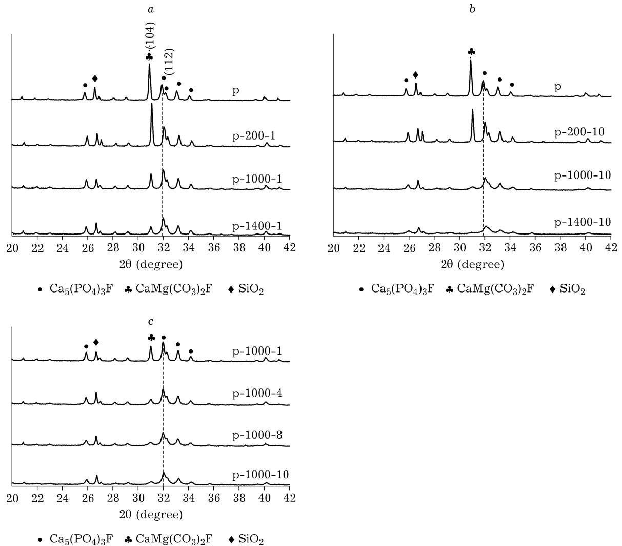
Fig. 2. XRD patterns of activated phosphate ore: a – one time, b – ten times, c – 1000 r/min.
