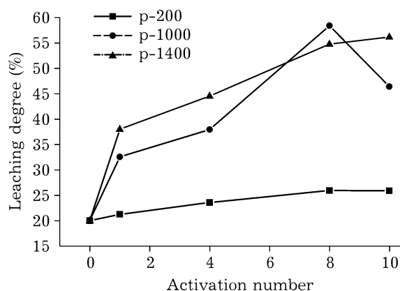
Fig. 4. Effect of activated phosphate ore on the leaching degree of available phosphorus.
