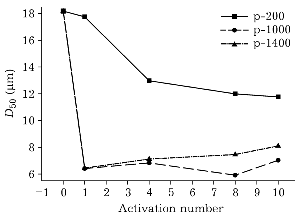
Fig. 1. Median diameter ( D_{50} ) distribution map of activated phosphate ore.
