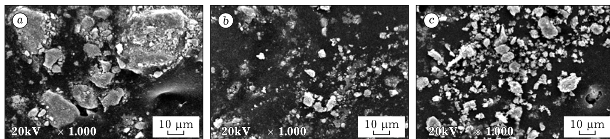
Fig. 3. SEM images of phosphate ore activated once (r/min): a – 200, b – 1000, c – 1400.
