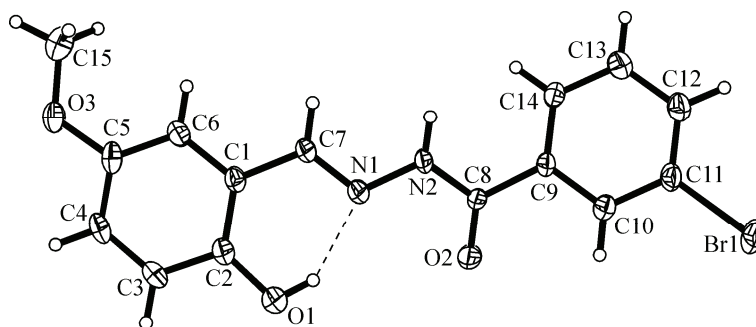
Fig. 1. Anisotropic ellipsoid representation of compound 1 together with the atom labeling scheme.
