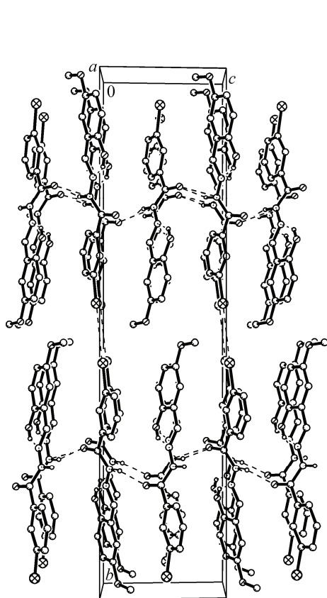
Fig. 3. Molecular packing diagram of 1 as seen along the a direction. Hydrogen bonds are shown as dashed lines
