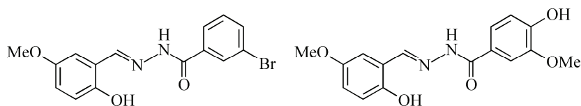
Scheme 1. Aroylhydrazones
