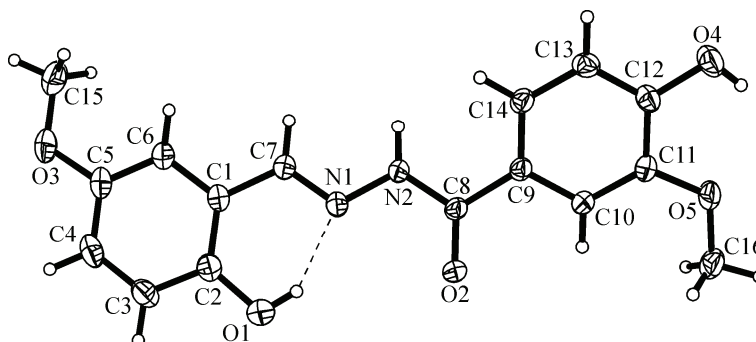
Fig. 2. Anisotropic ellipsoid representation of compound 2 together with the atom labeling scheme.
