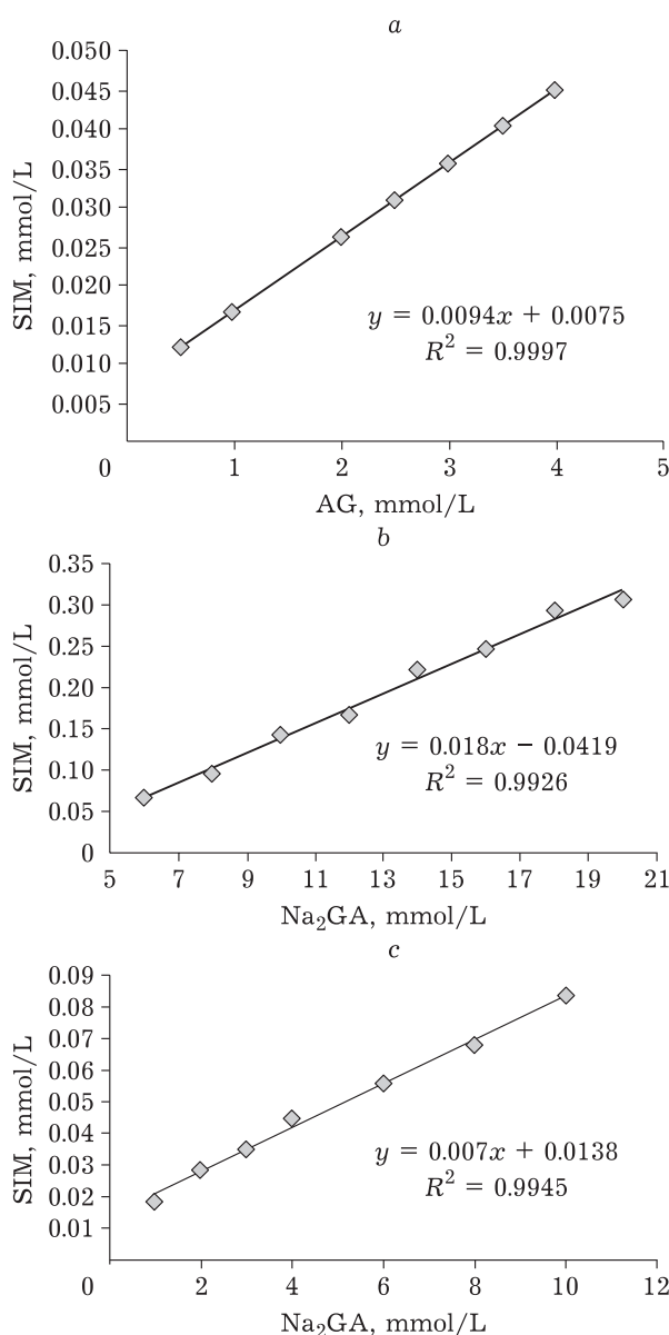
Fig. 5. Phase solubility diagrams of complexes simvastatin: SIM/AG (1 : 10, mass relations), SIM/ \text{Na}_2\text{GA} (1 : 2, mass relations) and SIM/ \text{Na}_2\text{GA} (1 : 4, mass relations) at 37 °C in aqueous solution [13] and calculated stability constants.
