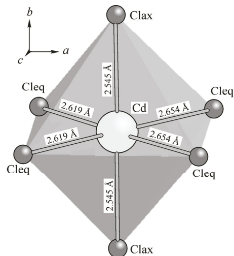
Fig. 4. View along c axis of the \text{CdCl}_6 octahedron
